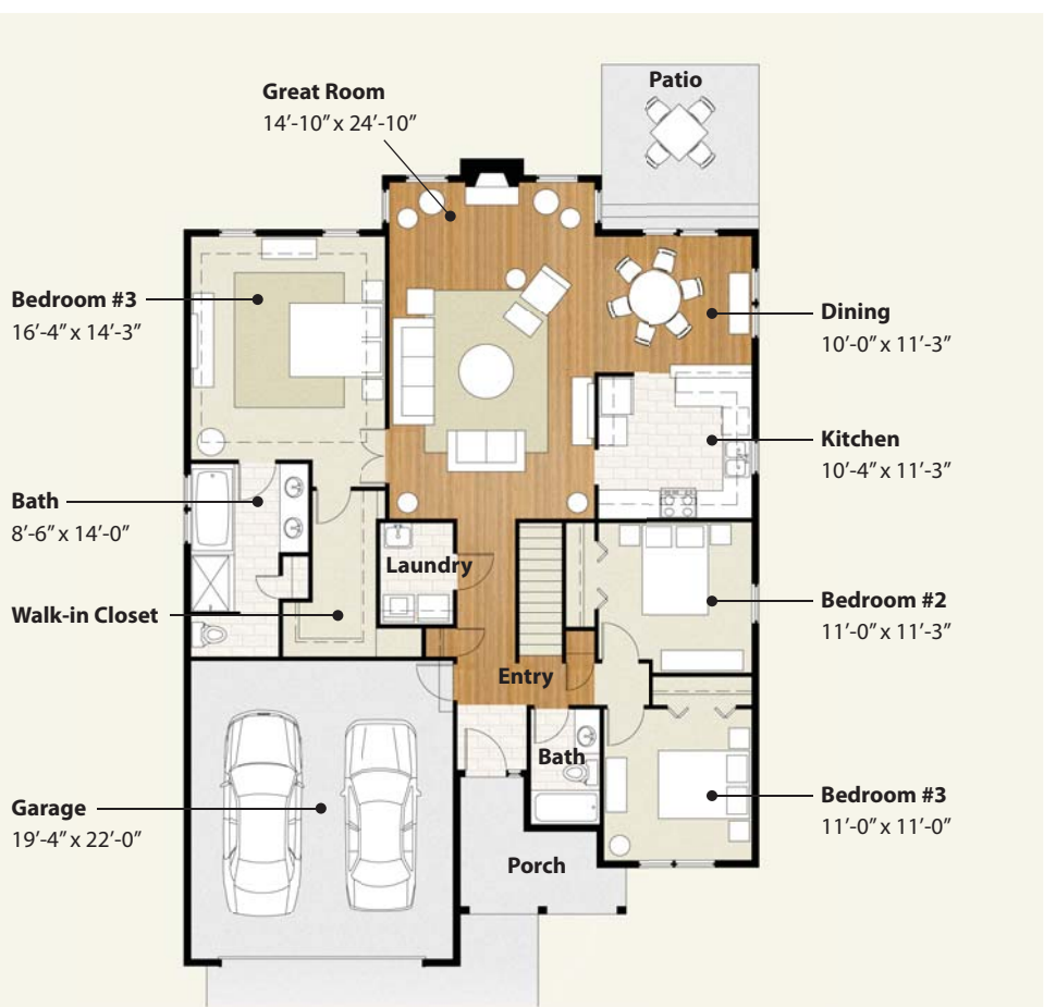
FLOOR PLAN
